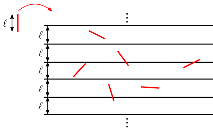
Figure 5: Buffon's Needle.
